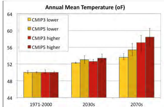
Figure 4. Historical and projected future annual mean temperature, based on the average of three long-term weather stations shown in Figure 3. Yellow bars show projected changes under lower scenarios and red bars, under higher. CMIP3 are the older generation of global climate models, and CMIP5 are the newer generation. The ranges on each bar show the projections from all the different models in each group (4 models in CMIP3 and 6 models in CMIP5).
