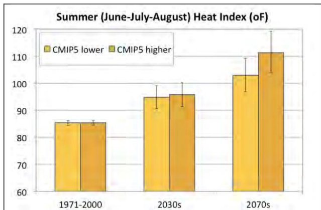
Figure 6. Historical and projected future summer heat index, based on projections for Boston Logan weather station (the nearest weather station with long-term humidity observations). Lighter gold bars show projected changes under lower scenarios and dark gold bars, under higher. Projections here are based on 8 CMIP5 models, as most CMIP3 models and one CMIP5 model did not have daily relative humidity projections available.
